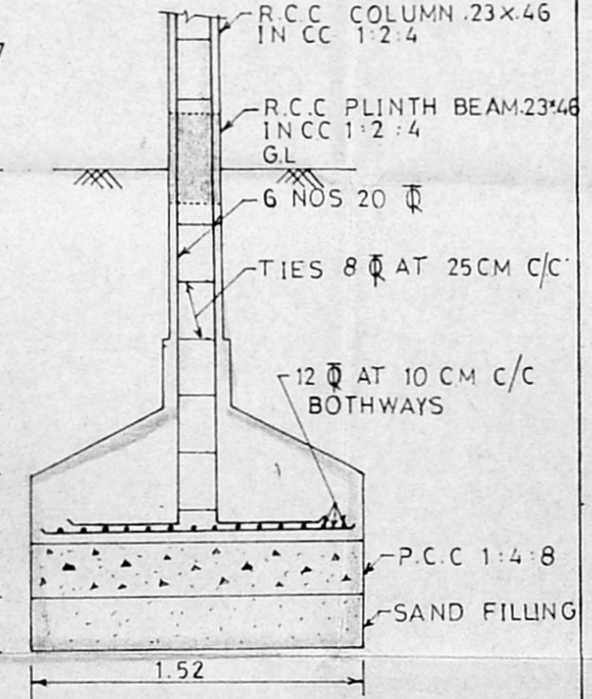
COLUMN FOUNDATION
